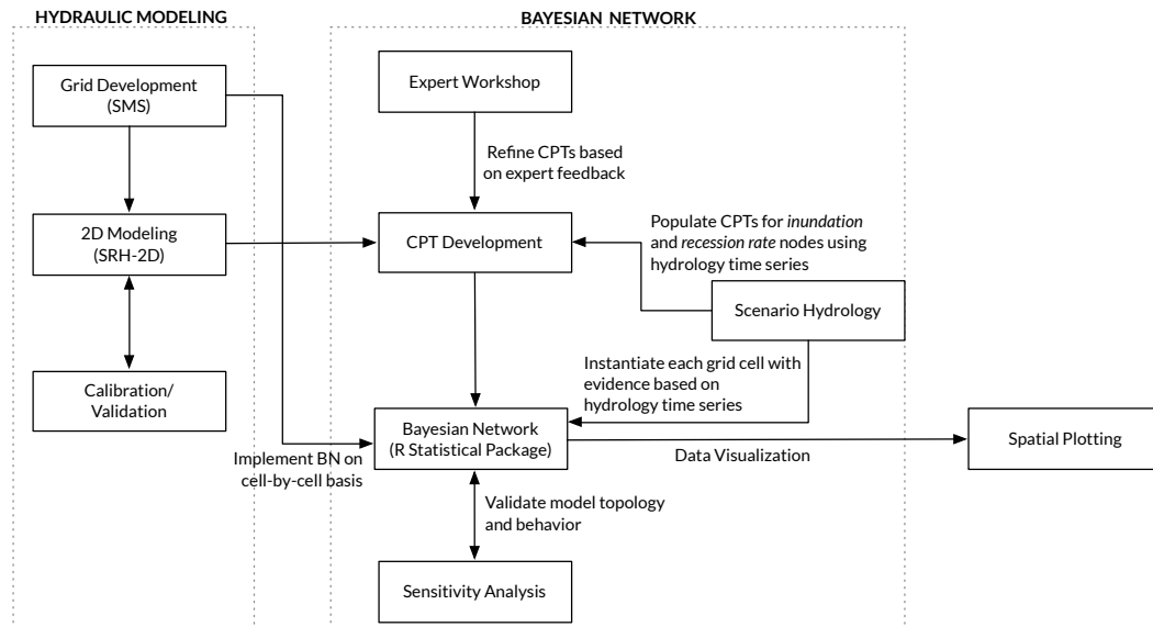
Figure 4.3: Schematic of modeling framework. Results from two-dimensional hydrodynamic modeling were used to instantiate the Bayesian network for each grid cell within each research site.
